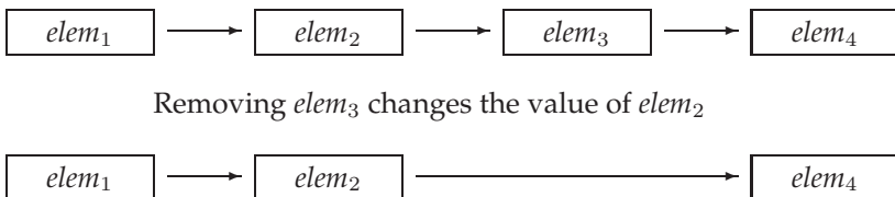
Figure 9.1: forward_list Specialized Operations
