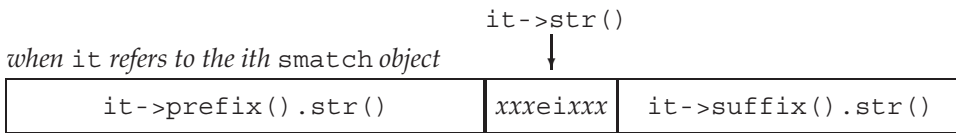
Figure 17.2: The smatch Object Representing a Particular Match
