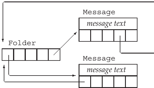
Figure 13.1: Message and Folder Class Design
