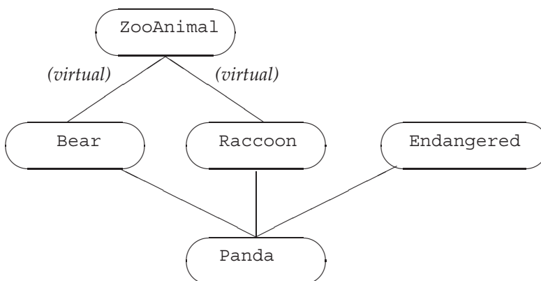
Figure 18.3: Virtual Inheritance Panda Hierarchy
