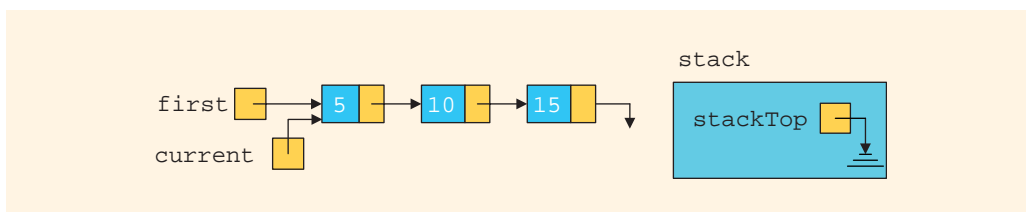
FIGURE 19-19 List after the statement current = first; executes
