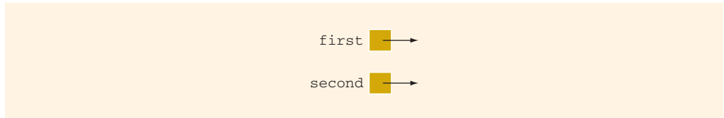
FIGURE 14-11 first and second after the statement delete [] second; executes
