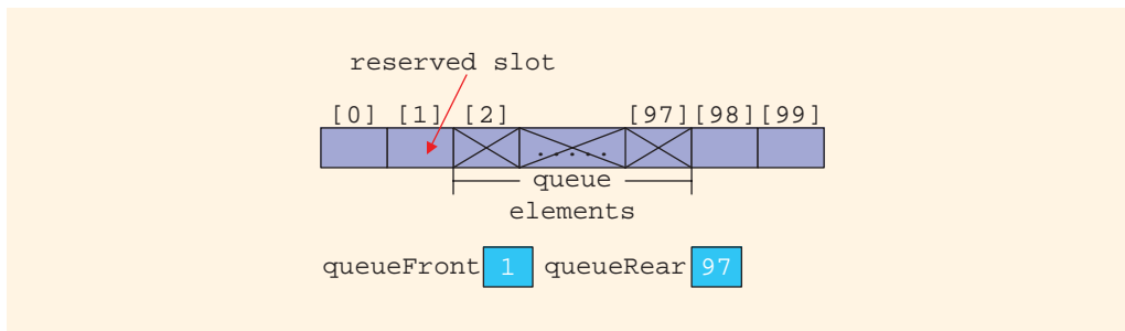
FIGURE 19-34 Array to store the queue elements with a reserved slot
