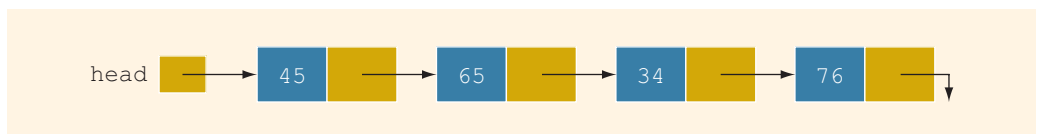
FIGURE 18-2 Linked list
