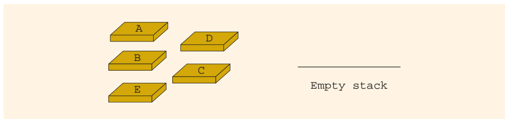
FIGURE 19-2 Empty stack
