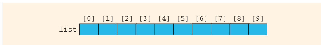
FIGURE 9-3 Array list
