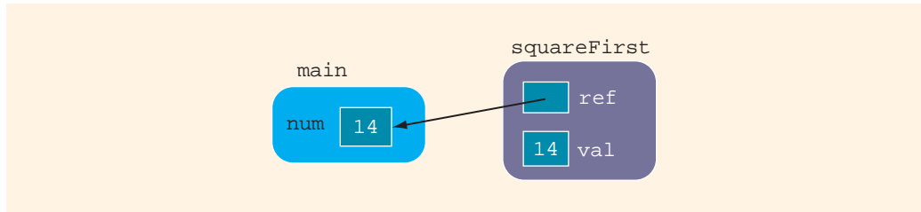
FIGURE 7-19 Parameters of the function squareFirst
