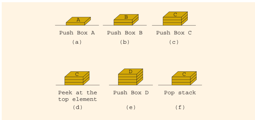
FIGURE 19-3 Stack operations
