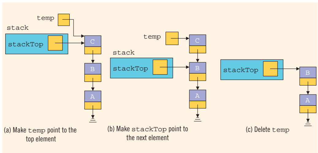
FIGURE 19-16 Pop operation
