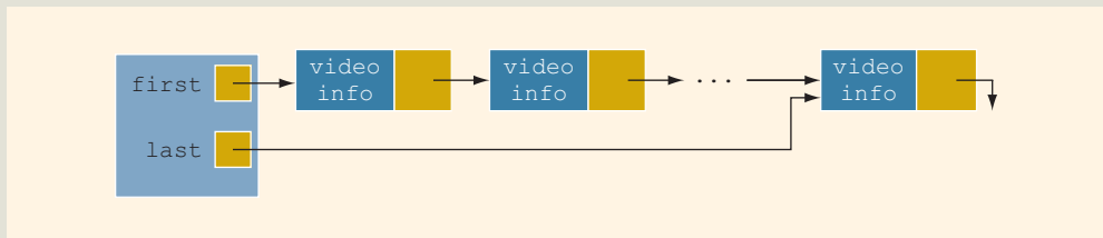
FIGURE 18-46 videoList
