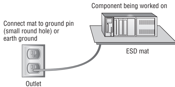
FIGURE 11.2 Proper use of an ESD antistatic mat
