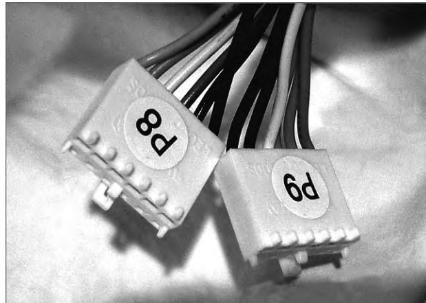
FIGURE 2.25 AT power supply system board connectors
