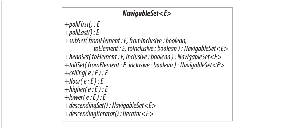
Figure 13-5. NavigableSet
