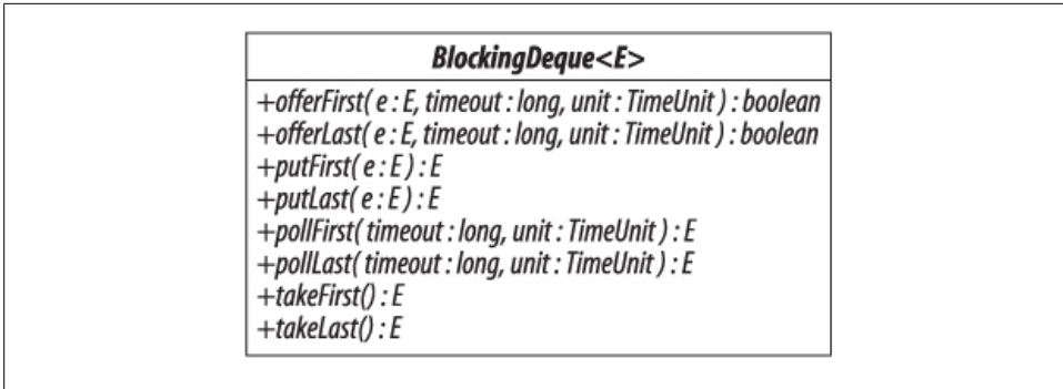
Figure 14-9. BlockingDeque
