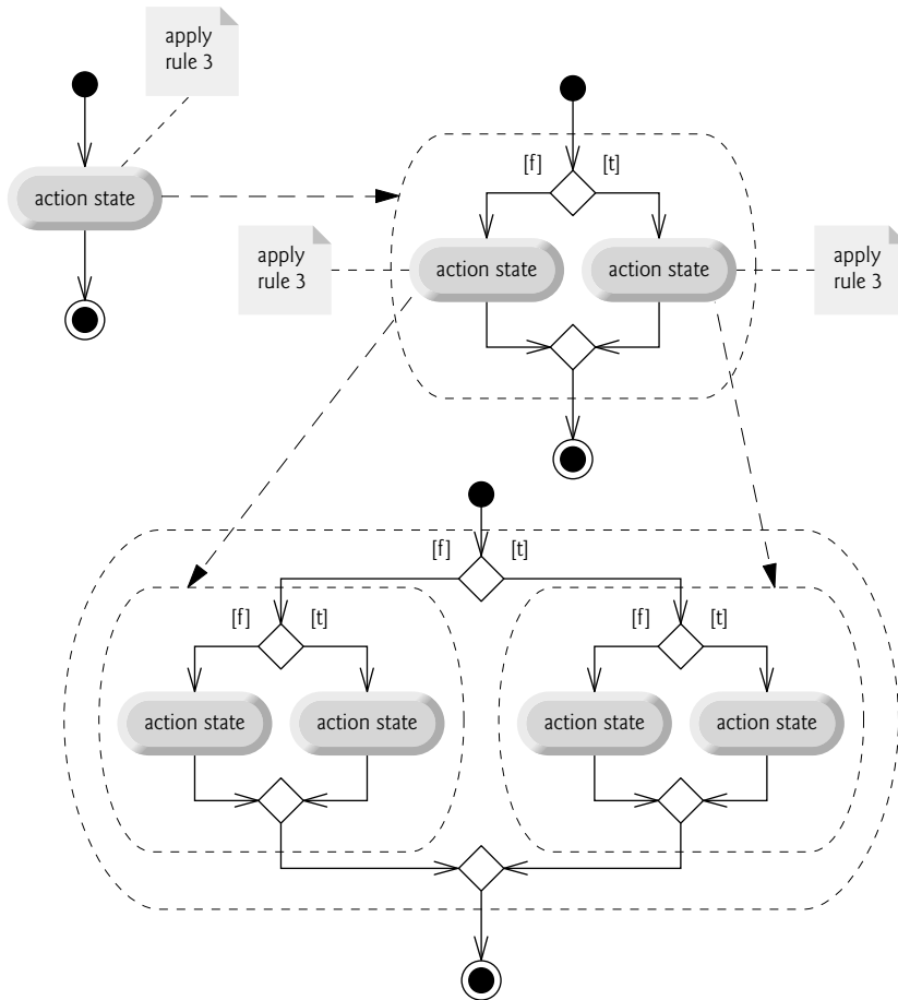
Fig. 4.23 | Repeatedly applying rule 3 of Fig. 4.20 to the simplest activity diagram.
