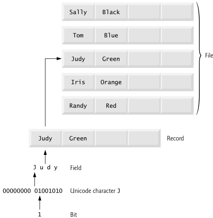
Fig. 1.3 | Data hierarchy.
