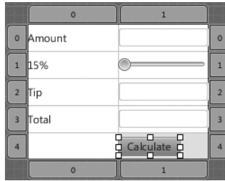
Fig. 25.13 | GridPane filled with the Tip Calculator’s controls.
