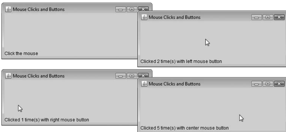
Fig. 12.32 | Testing MouseDetailsFrame.
