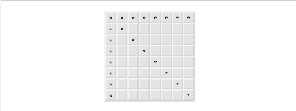
Fig. 6.24 | The 22 squares eliminated by placing a queen in the upper left corner.
