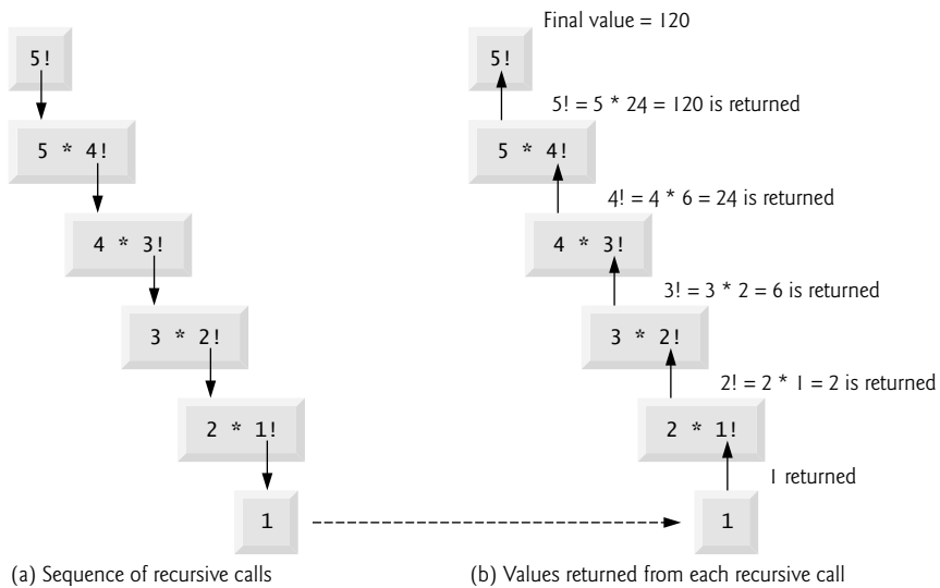
Fig. 18.2 | Recursive evaluation of 5!.
