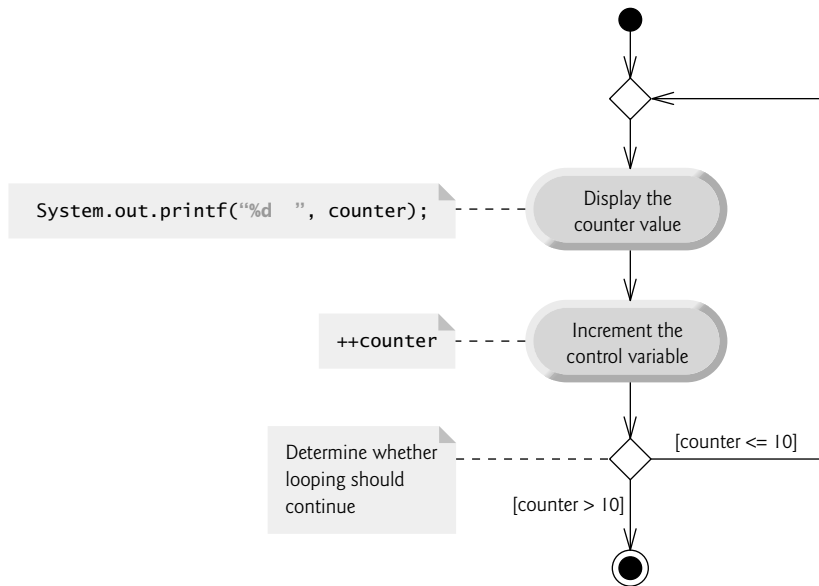
Fig. 4.8 | do...while repetition statement UML activity diagram.
