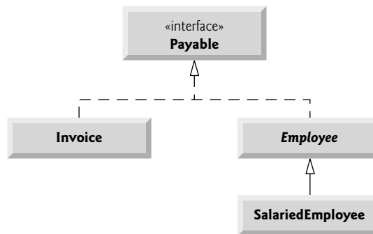
Fig. 10.10 | Payable hierarchy UML class diagram.
