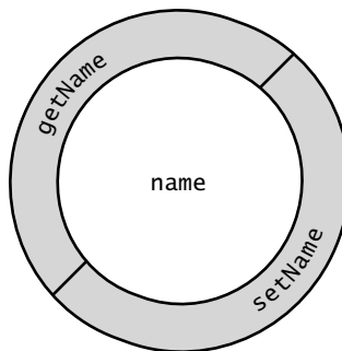
Fig. 7.4 | Conceptual view of an Account object with its encapsulated private instance variable name and protective layer of public methods.
