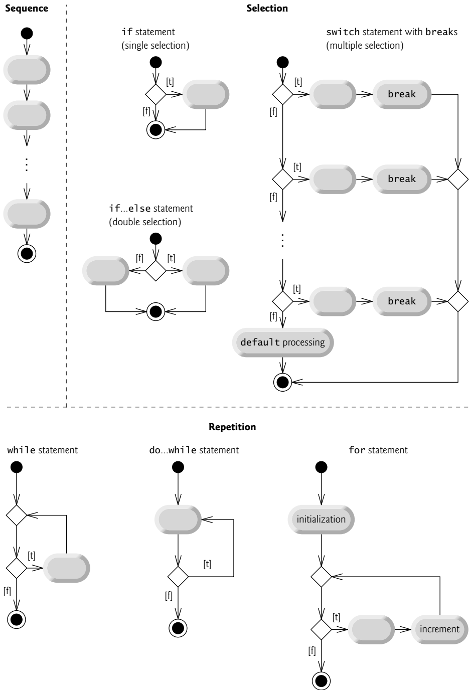
Fig. 4.19 | Java's single-entry/single-exit sequence, selection and repetition statements.
