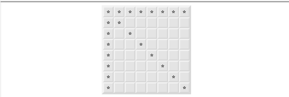
Fig. 18.20 | Squares eliminated by placing a queen in the upper-left corner of a chessboard.
