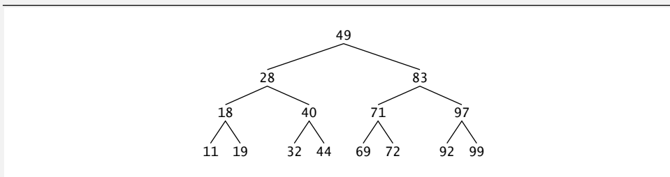
Fig. 21.20 | Binary search tree with 15 nodes.
