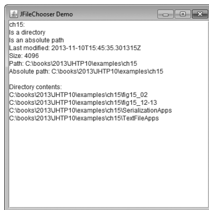
Fig. 15.13 | Testing class FileDemonstration. (Part 2 of 2.)
