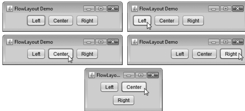
Fig. 12.40 | Testing FlowLayoutFrame.
