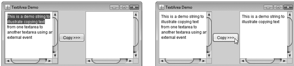
Fig. 12.48 | Testing TextAreaFrame.
