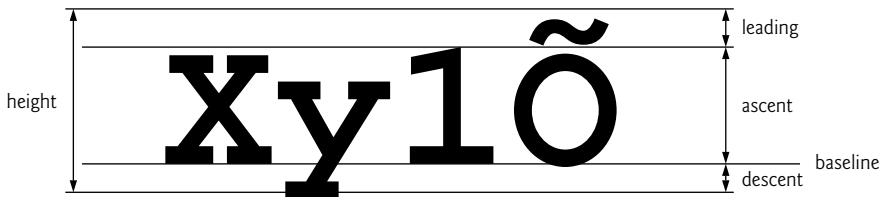
Fig. 13.13 | Font metrics.
