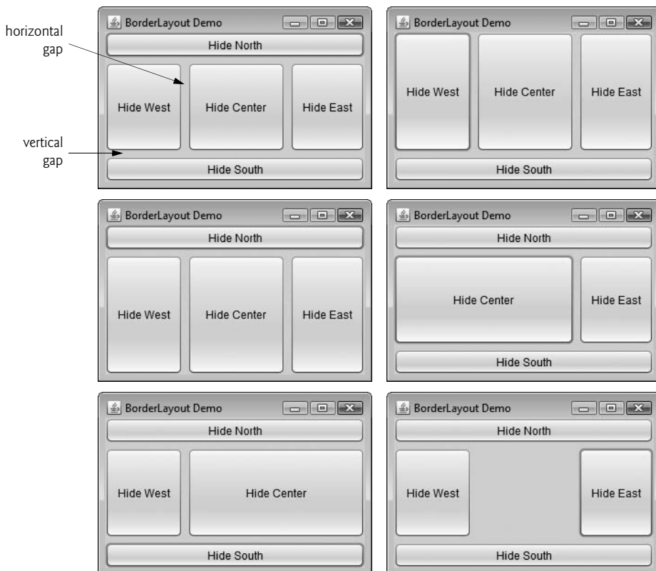
Fig. 12.42 | Testing BorderLayoutFrame .
