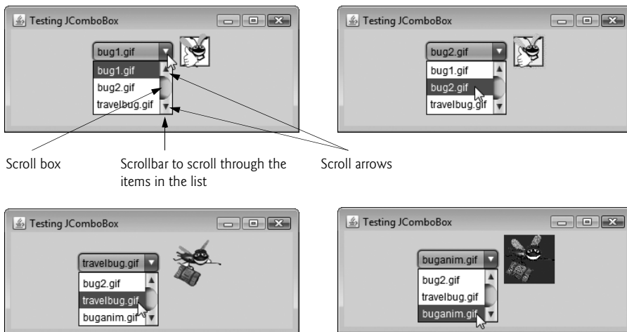
Fig. 12.22 | Testing ComboBoxFrame.
