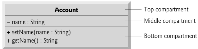
Fig. 7.3 | UML class diagram for class Account of Fig. 7.1.
