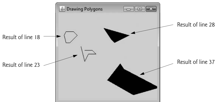
Fig. 13.28 | Drawing polygons.
