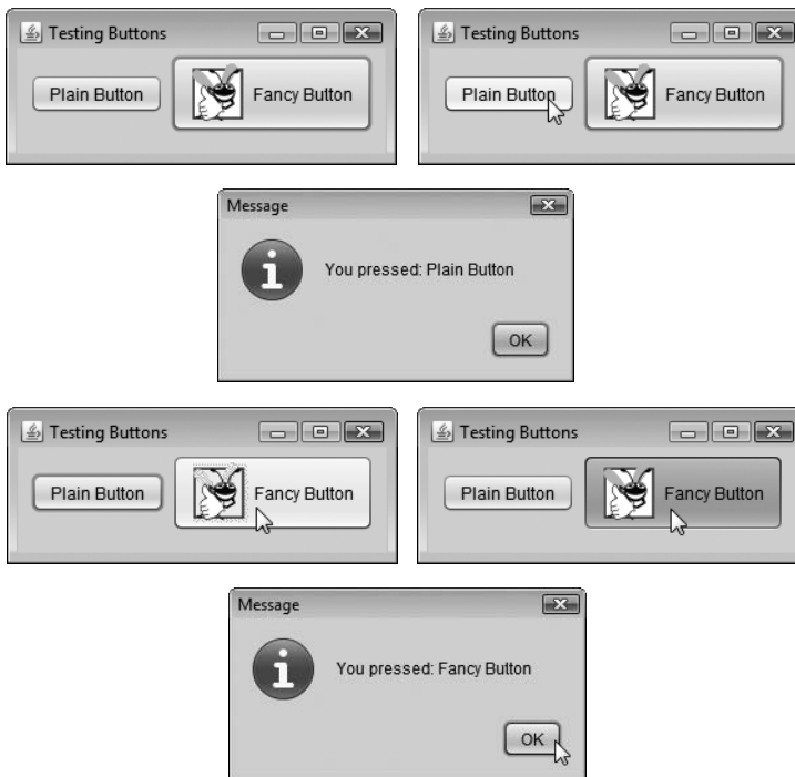
Fig. 12.16 | Testing ButtonFrame.
