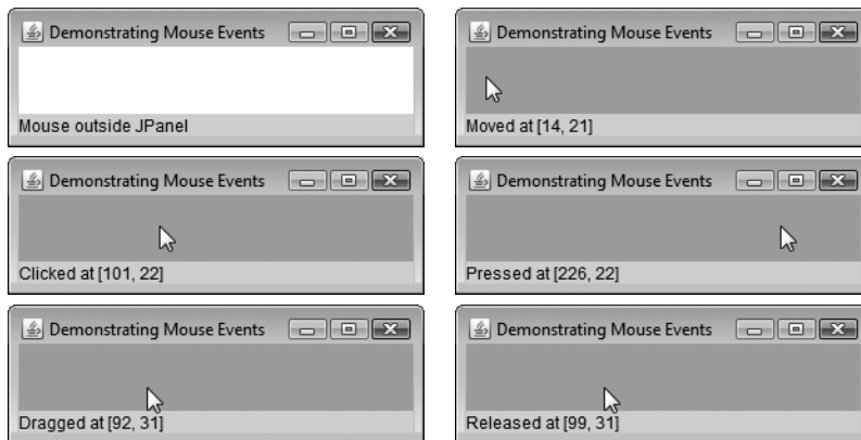
Fig. 12.29 | Testing MouseTrackerFrame.
