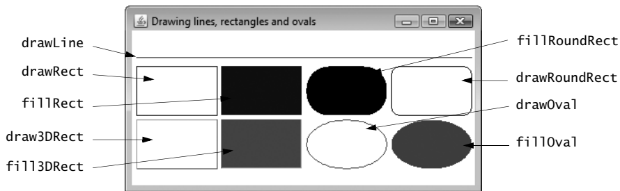
Fig. 13.19 | Testing LinesRectsOvalsJPanel.
