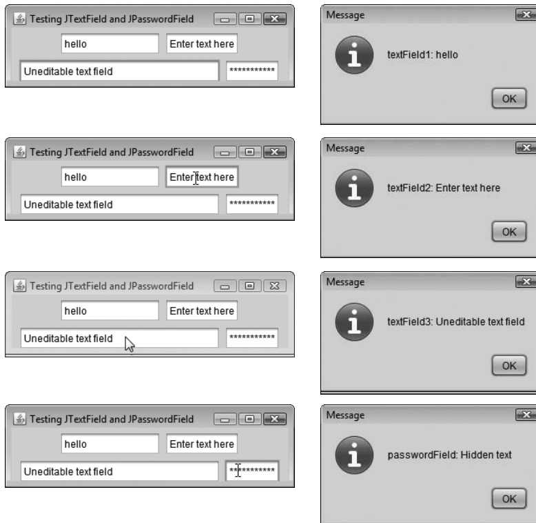
Fig. 12.10 | Testing TextFieldFrame. (Part 2 of 2.)
