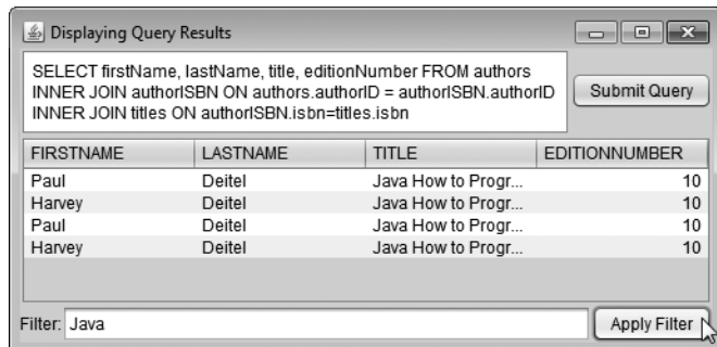
Fig. 24.28 | Display the contents of the Authors table in the books database. (Part 5 of 5.)
