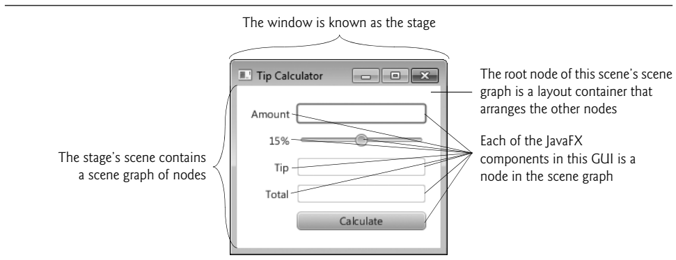
Fig. 25.1 | JavaFX app window parts.
