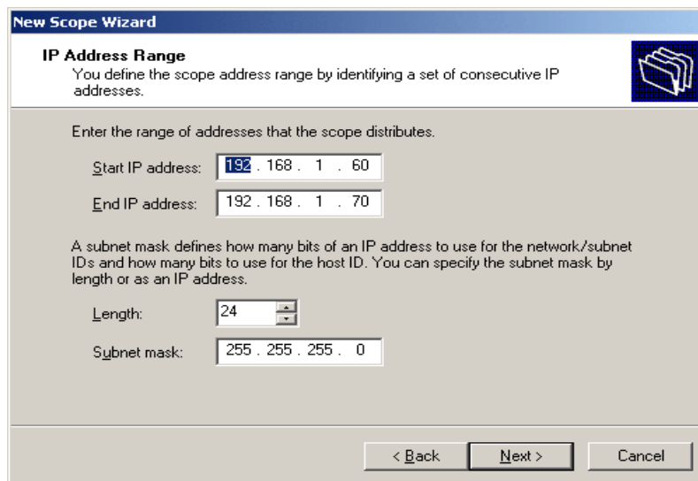
Gambar 1.4 Tampilan DCHP Server
