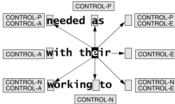
Figure 7-6 Moving the cursor by lines
