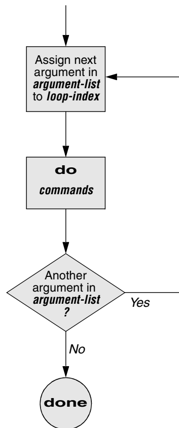
Figure 10-4 A for...in flowchart
