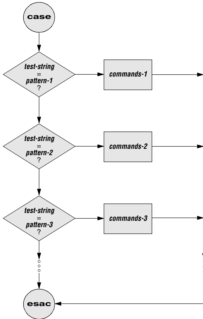
Figure 10-7 A case flowchart
