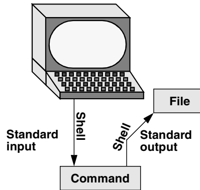
Figure 5-6 Redirecting standard output
