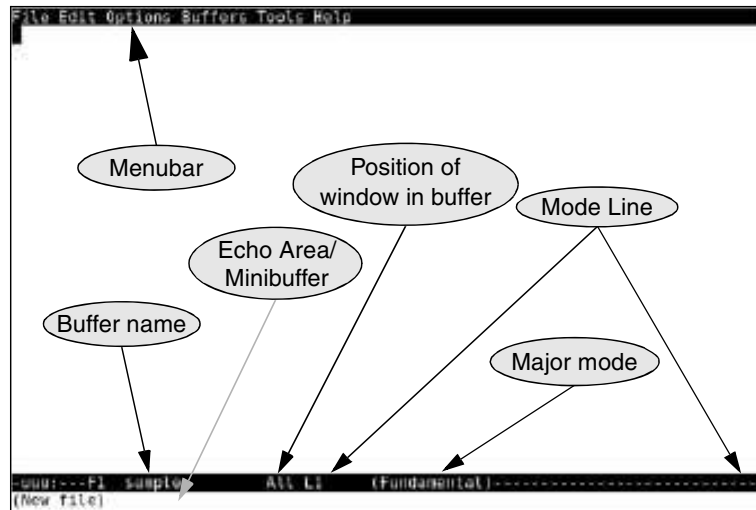
Figure 7-1 The emacs new file screen
