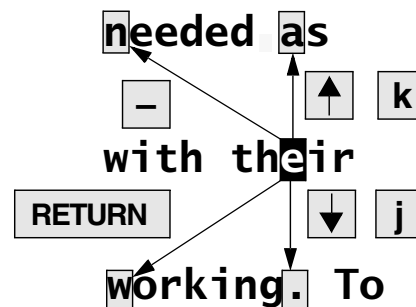
Figure 6-11 Moving the cursor by lines
