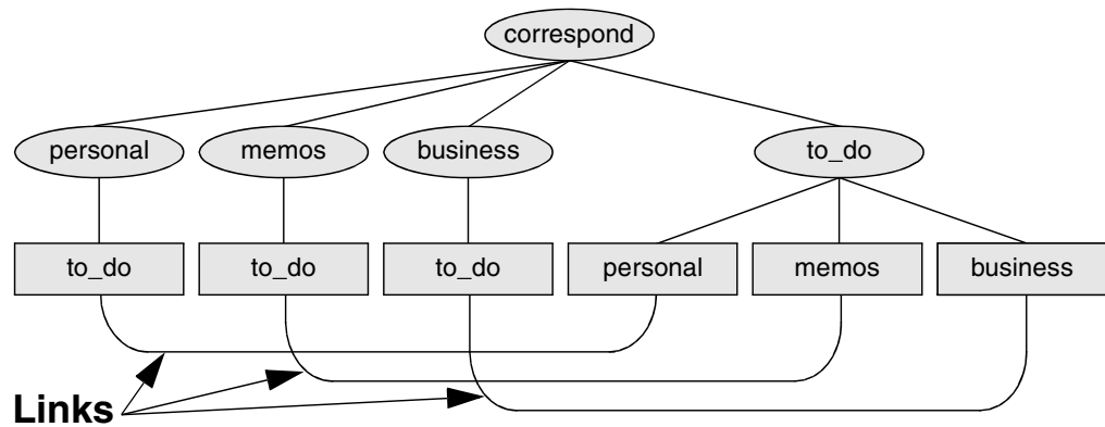
Figure 4-13 Using links to cross-classify files
