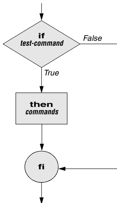
Figure 10-1 An if...then flowchart
