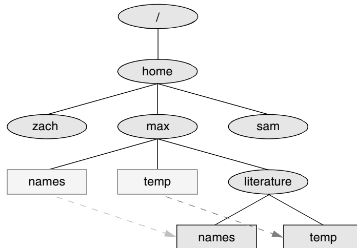
Figure 4-10 Using mv to move names and temp
