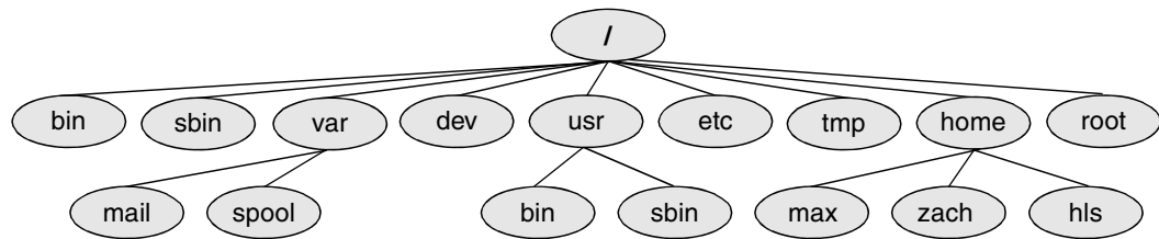
Figure 4-11 A typical FHS-based Linux filesystem structure
