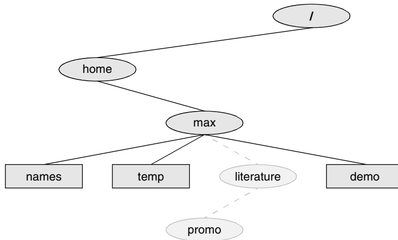
Figure 4-7 The file structure developed in the examples
