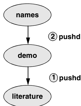
Figure 8-3 Creating a directory stack
