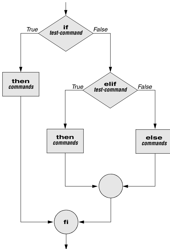
Figure 10-3 An if...then...elif flowchart
