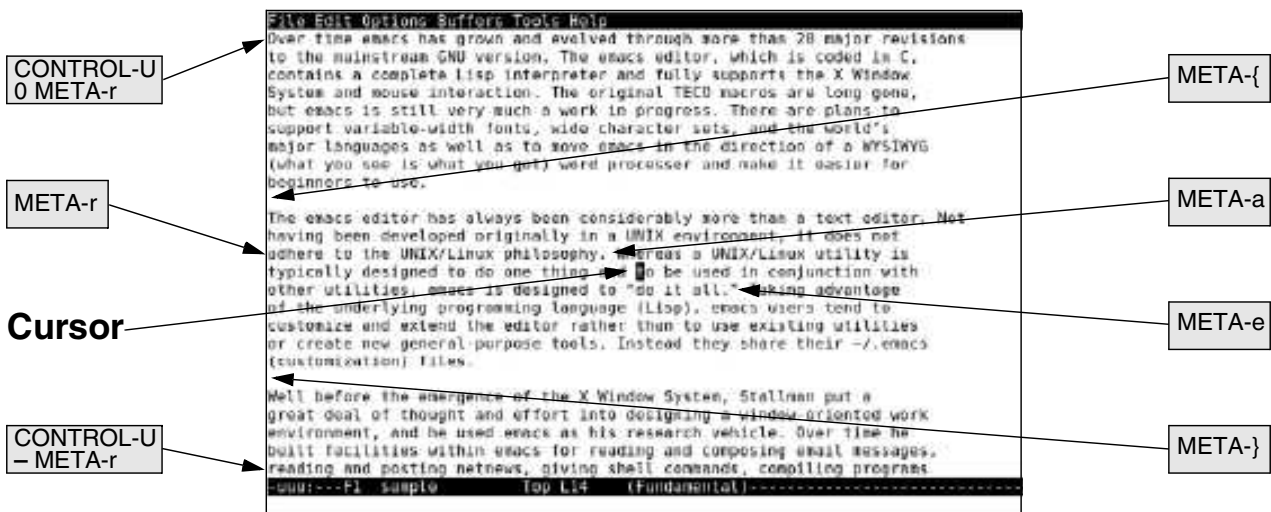
Figure 7-7 Moving the cursor by sentences, paragraphs, and window position
