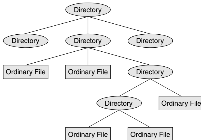
Figure 4-3 Directories and ordinary files
