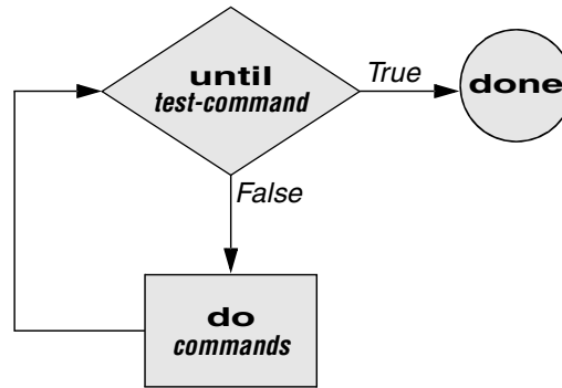
Figure 10-6 An until flowchart
