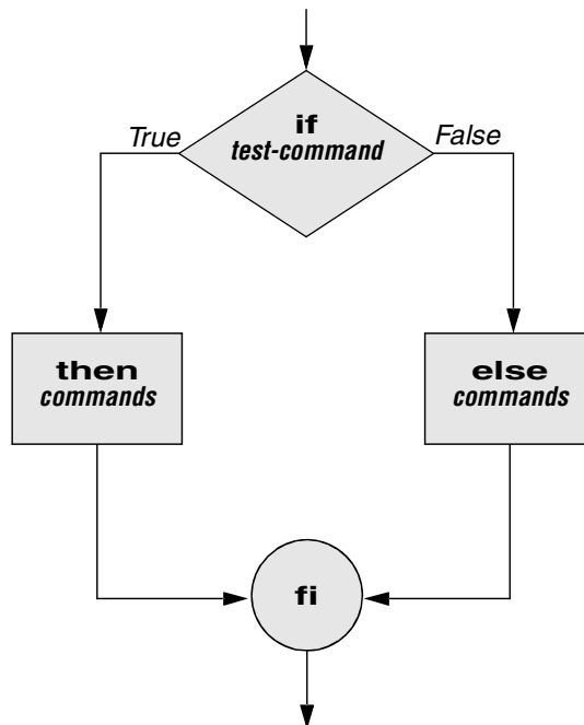
Figure 10-2 An if...then...else flowchart
