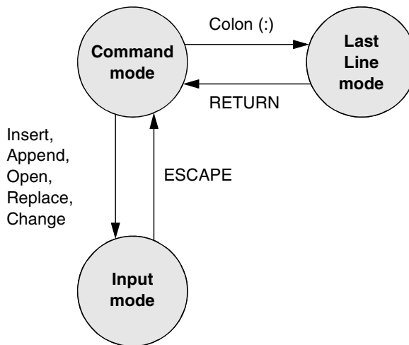
Figure 6-3 Modes in vim
