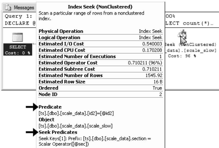
Figure 3.3. Predicate Information as a Tool Tip
