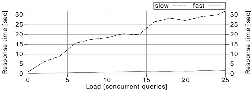
Figure 3.4. Scalability by System Load
