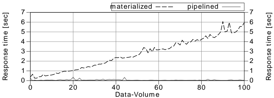
Figure 7.1. Scalability of Top-N Queries
