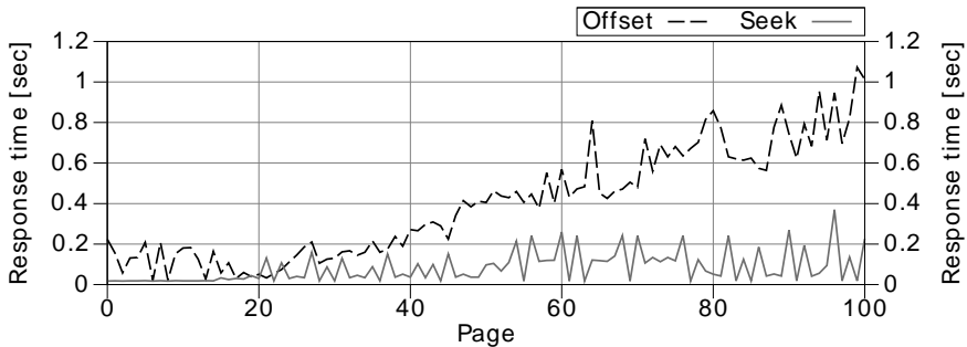
Figure 7.4. Scalability when Fetching the Next Page
